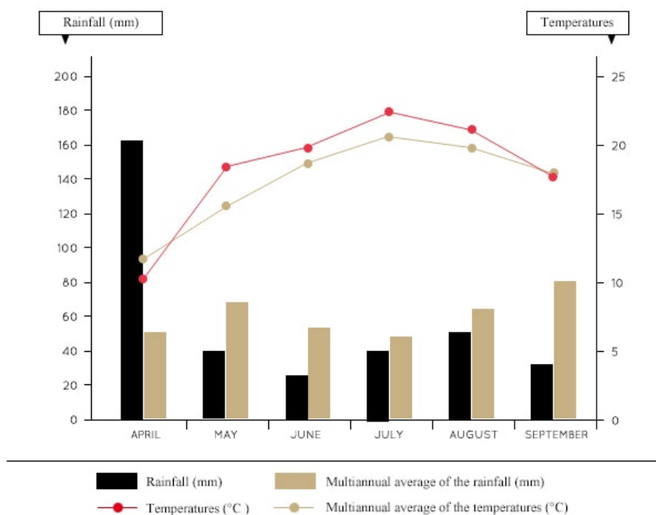
1989 : TEMPERATURES AND RAINFALL COMPARED WITH NORMAL VALUES IN SAINT-EMILION
